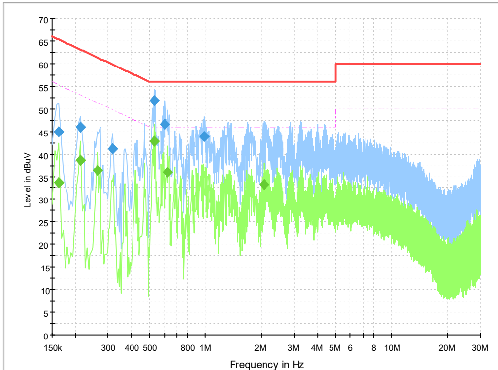
Fig.B.11.1 AC Powerline Conducted Emission- bluetooth
