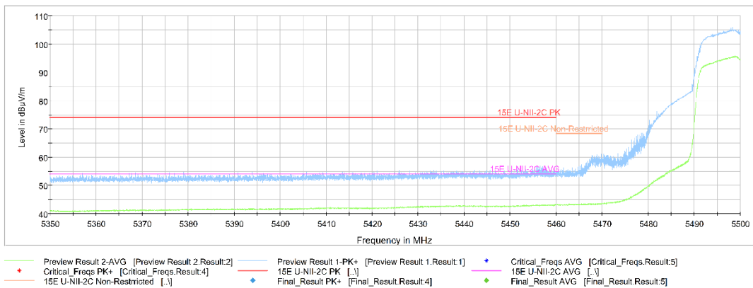
Fig.44 Band Edges (802.11n-HT40 Ch102, 5510MHz)
