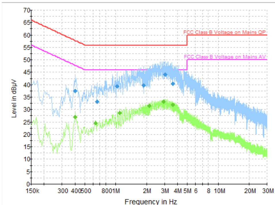
Fig.B.9.2 AC Powerline Conducted Emission-Idle
