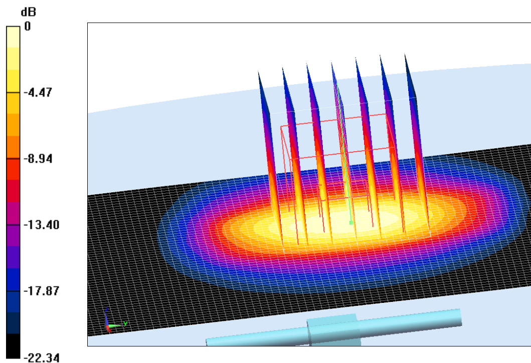
Fig.B.4 validation 2450 MHz 250mW
