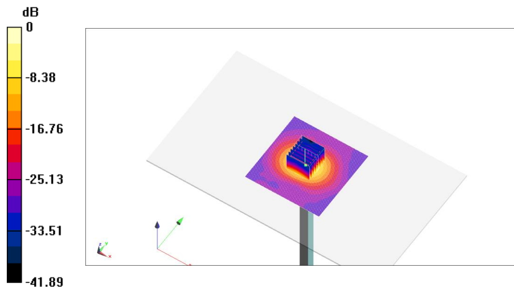
Fig.B.7 validation 5600 MHz 100mW
