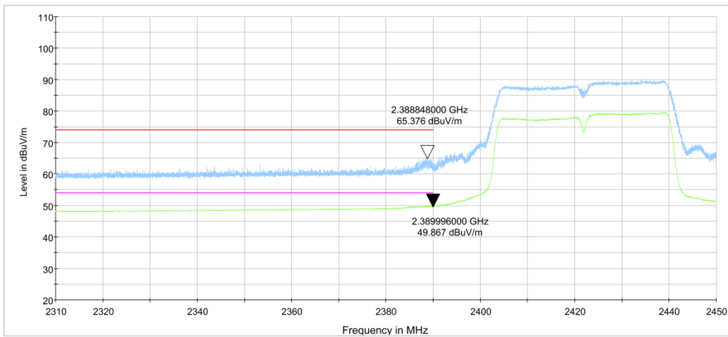
Fig.A.6.2.7 Transmitter Spurious Emission - Radiated (Power): 802.11n-HT40, ch3, 2.31 GHz - 2.45GHz
