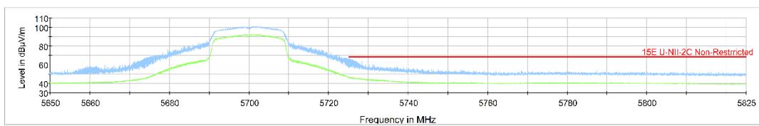
Fig.41 Band Edges (802.11n-HT20 Ch140, 5700MHz)
