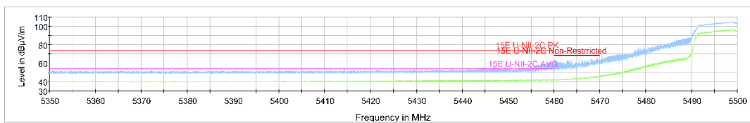
Fig.40 Band Edges (802.11n-HT20 Ch100, 5500MHz)
