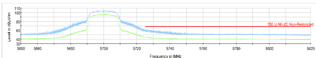
Fig.37 Band Edges (802.11a Ch140, 5700MHz)
