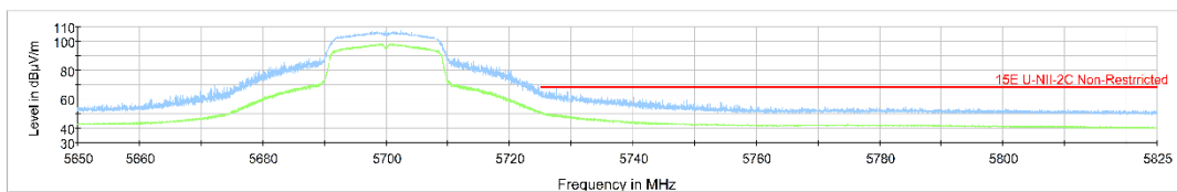
Fig.49 Band Edges (802.11ac-HT20 Ch140, 5700MHz)
