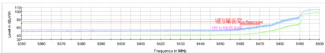
Fig.36 Band Edges (802.11a Ch100, 5500MHz)
