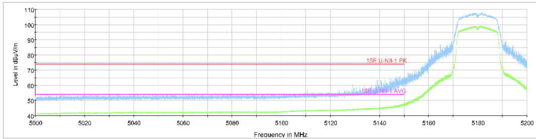
Fig.34 Band Edges (802.11a Ch36, 5180MHz)
