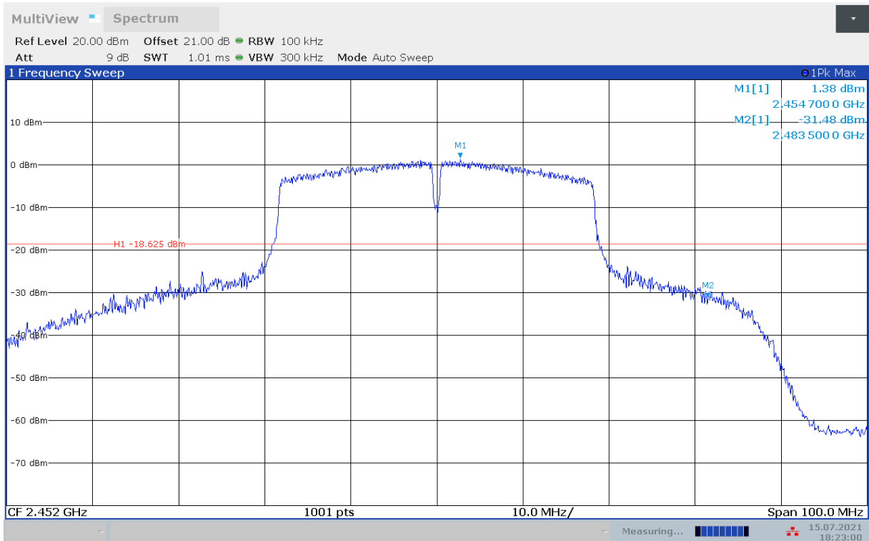
Fig.A.6.1.23 Transmitter Spurious Emission - Conducted (802.11n-HT40, Ch9, Center Frequency)
