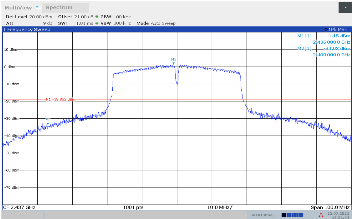
Fig.A.6.1.21 Transmitter Spurious Emission - Conducted (802.11n-HT40, Ch6, Center Frequency)
