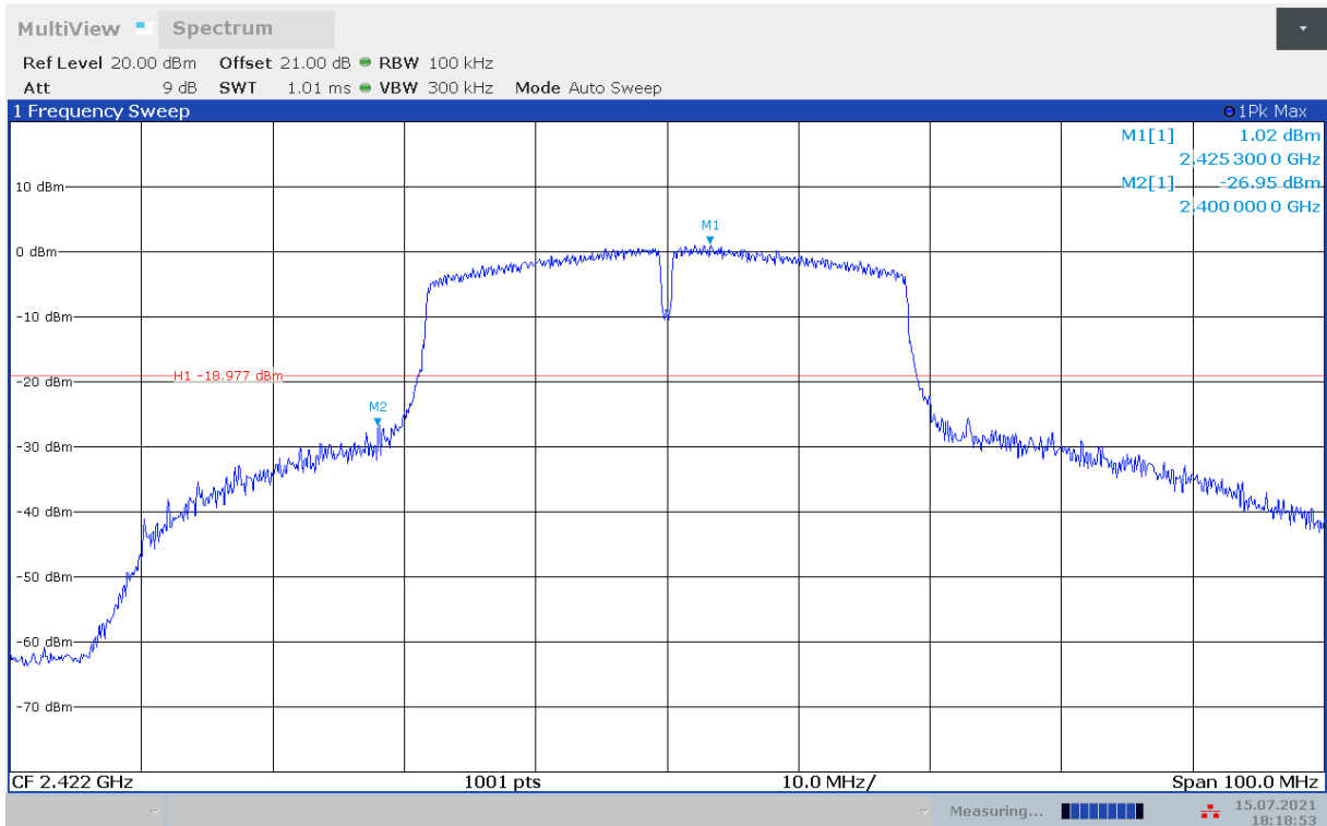
Fig.A.6.1.19 Transmitter Spurious Emission - Conducted (802.11n-HT40, Ch3, Center Frequency)
