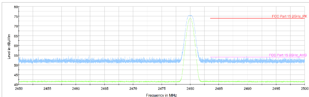
Fig.4. Frequency Band Edges: GFSK, 2480 MHz, Hopping Off , 2.45 GHz - 2.50GHz
