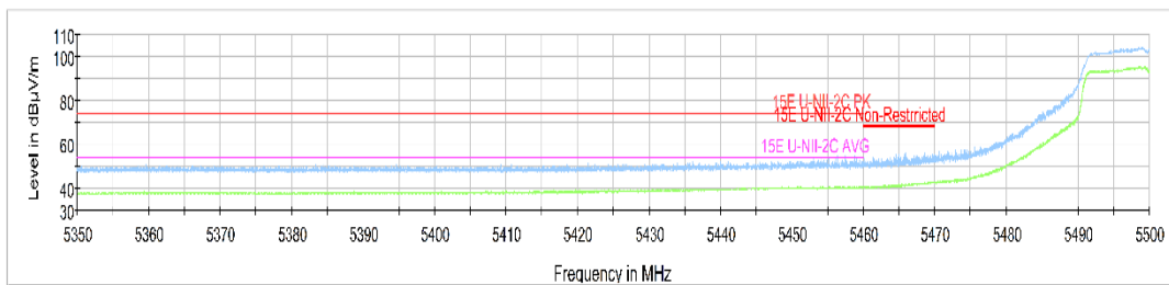
Fig.40 Band Edges (802.11n-HT20 Ch100, 5500MHz)
