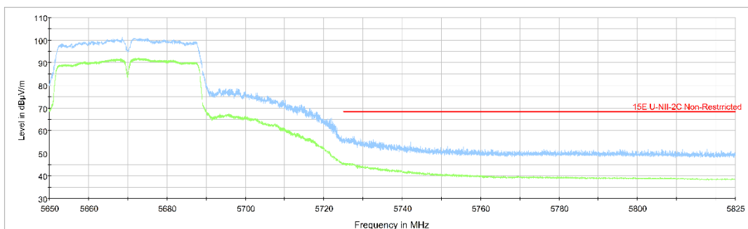
Fig.45 Band Edges (802.11n-HT40 Ch134, 5670MHz)
