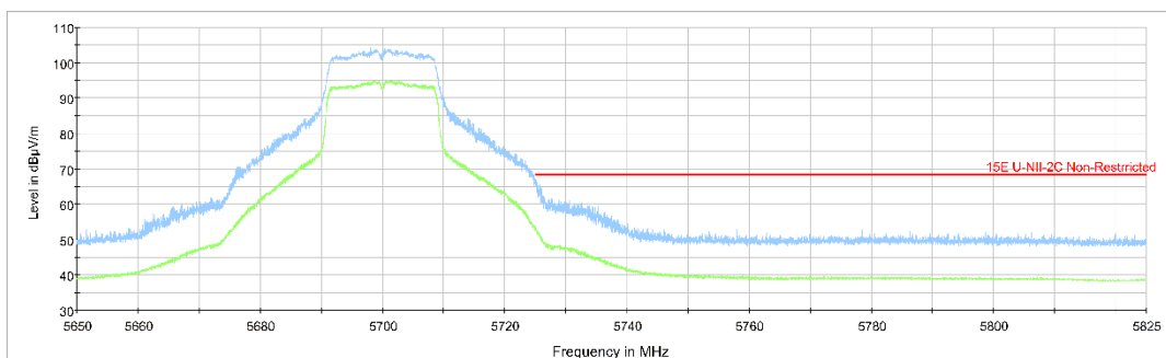
Fig.49 Band Edges (802.11ac-HT20 Ch140, 5700MHz)
