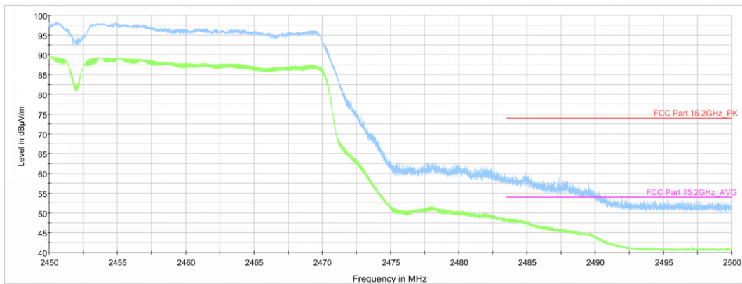
Fig.A.6.2.8 Transmitter Spurious Emission - Radiated (Power): 802.11n-HT40, ch9, 2.45 GHz - 2.50GHz
