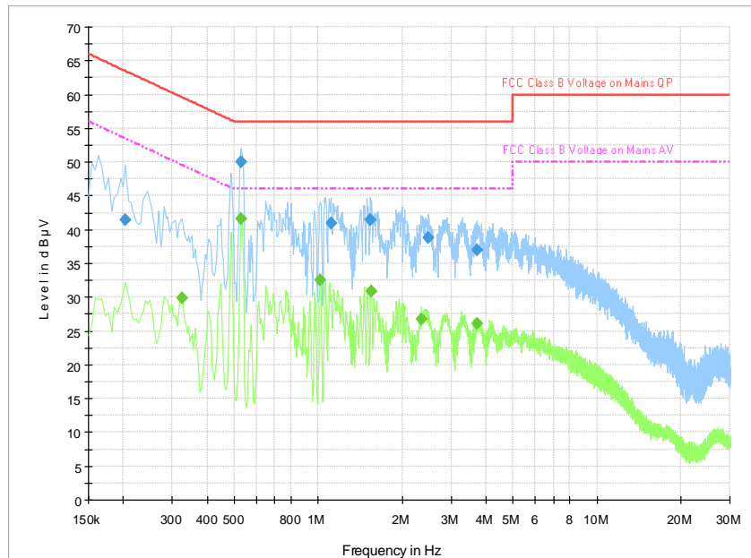
Fig.B.11.4 AC Powerline Conducted Emission- bluetooth
