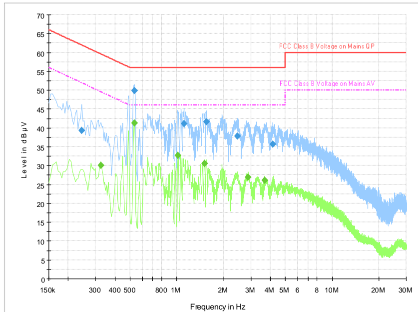
Fig.B.11.3 AC Powerline Conducted Emission- bluetooth
