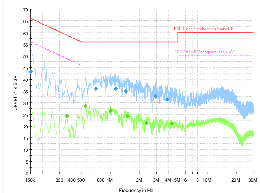
Fig.B.11.2 AC Powerline Conducted Emission- bluetooth
