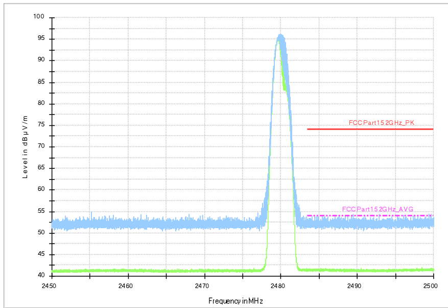
Fig.18. Frequency Band Edges: 8DPSK, Channel 78, 2.45 GHz - 2.50GHz
