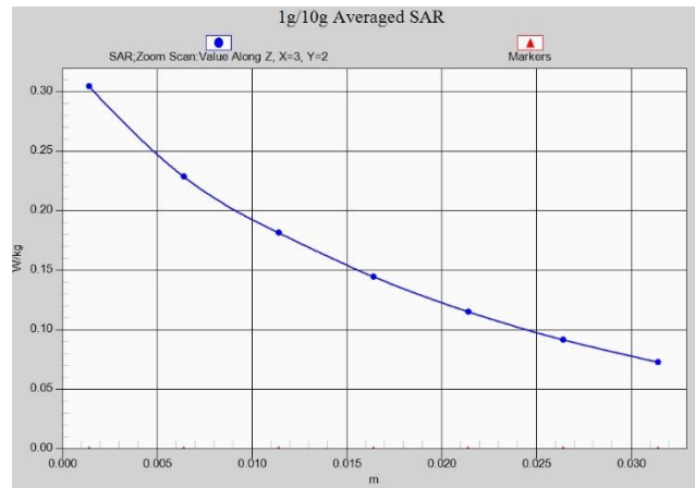
Fig. 1-10 Z-Scan at power reference point (LTE Band5)
