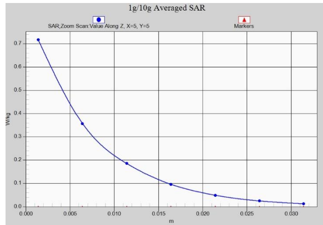
Fig. 1-16 Z-Scan at power reference point (wifi2450)
