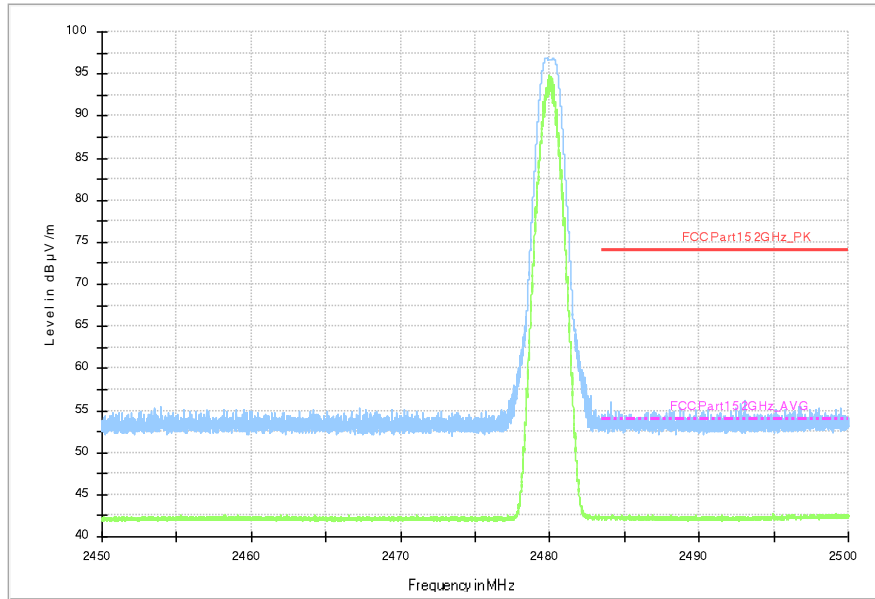
Fig.4. Frequency Band Edges: GFSK, 2480 MHz, 2.45 GHz - 2.50GHz
