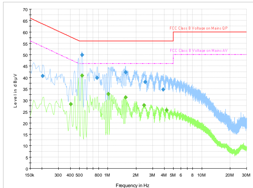
Fig.B.9.4 AC Powerline Conducted Emission-Idle
