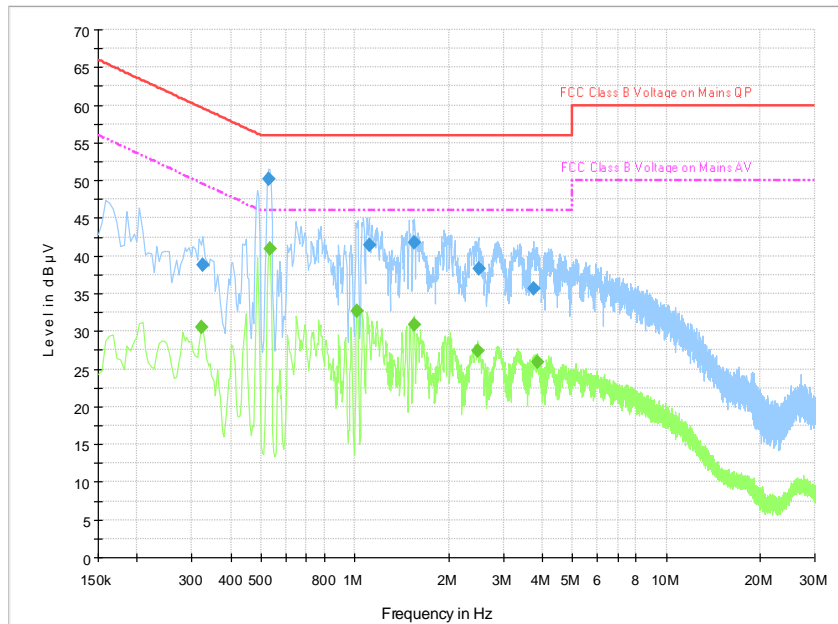
Fig.B.9.3 AC Powerline Conducted Emission-Idle
