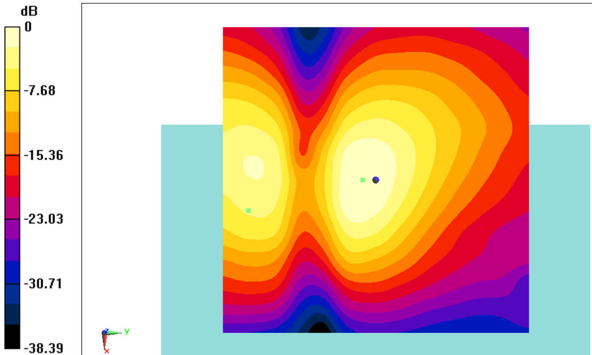
Fig B.3 T-Coil LTE B26
