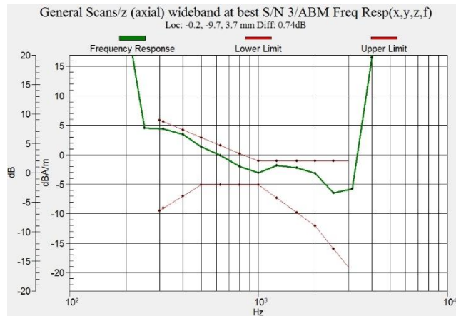
Figure C.2 Frequency Response of LTE B13
