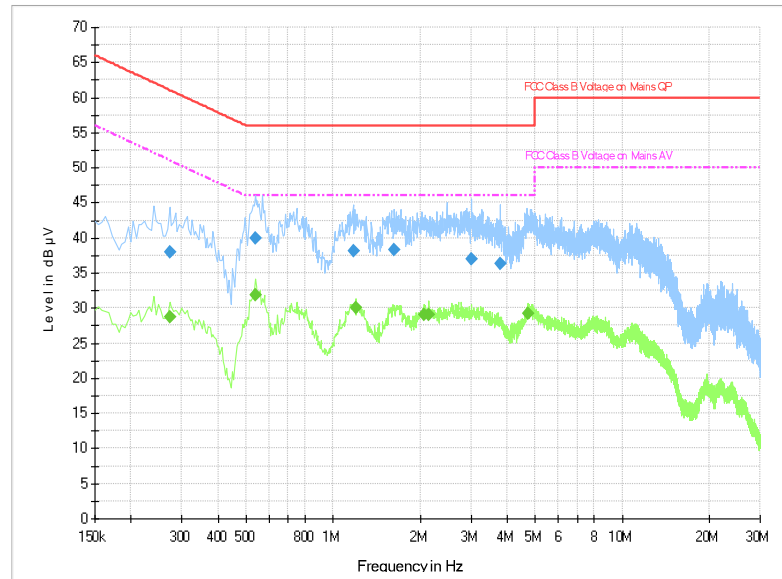
Fig.B.9.2 AC Powerline Conducted Emission-Idle
