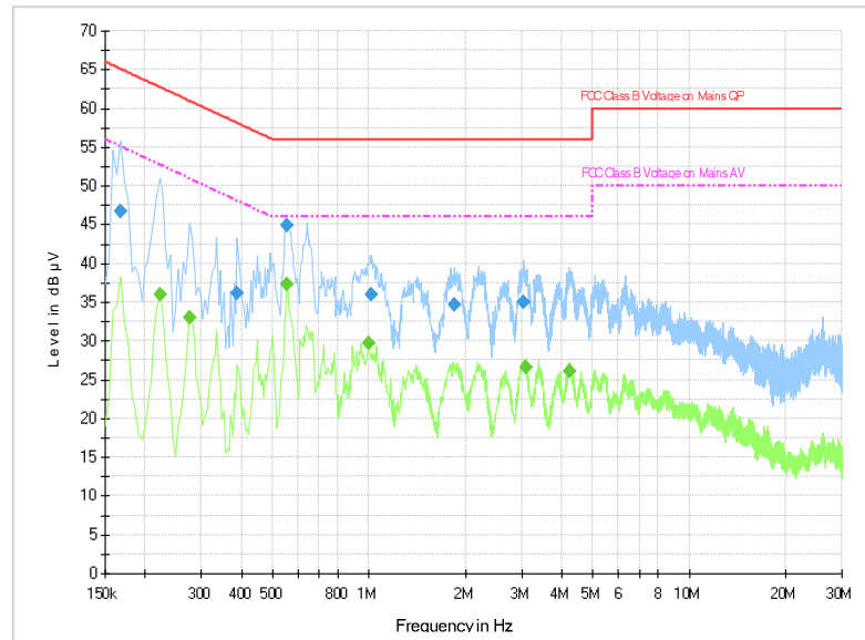
Fig.B.9.1 AC Powerline Conducted Emission-traffic
