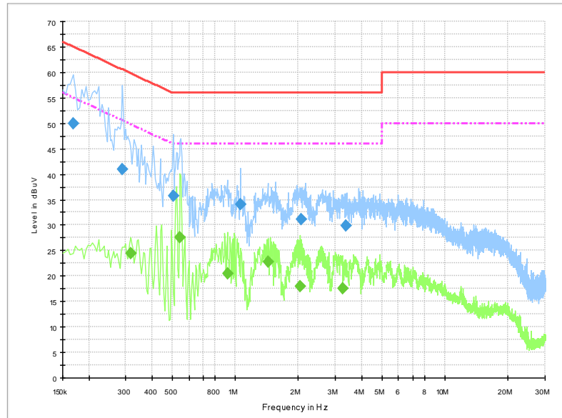
Fig.B.9.1 AC Powerline Conducted Emission-traffic
