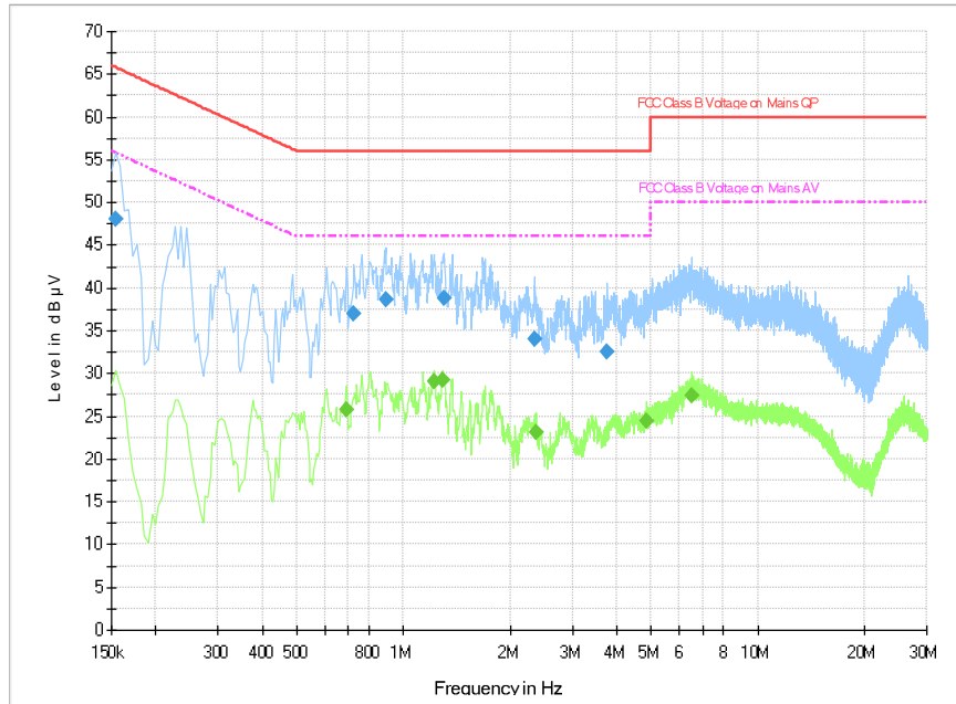
Fig.B.9.1 AC Powerline Conducted Emission- bluetooth
