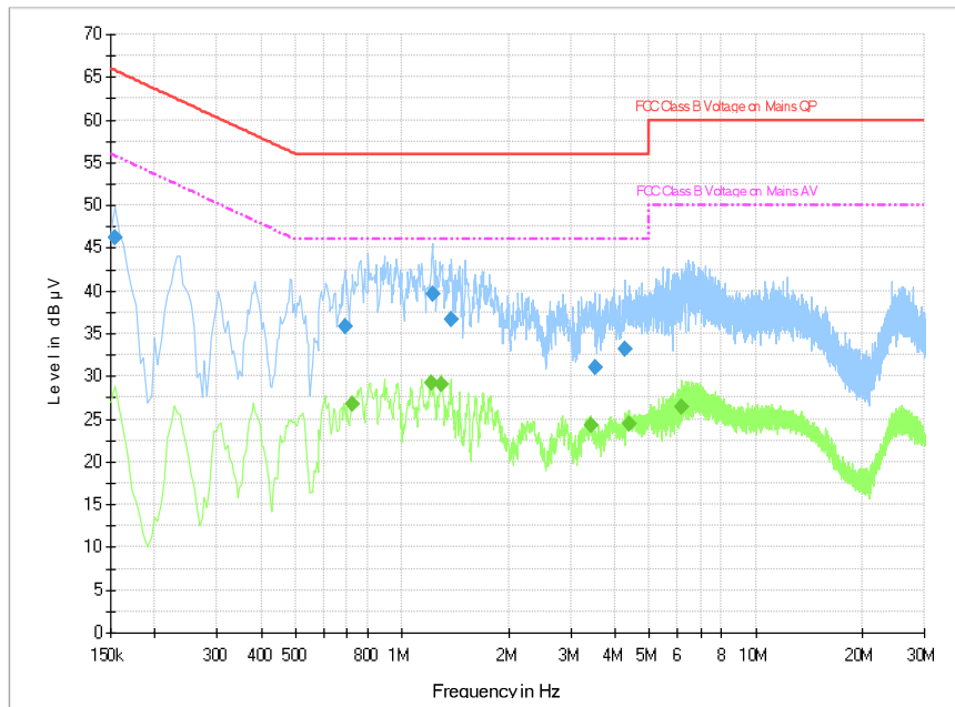
Fig.B.9.2 AC Powerline Conducted Emission-Idle
