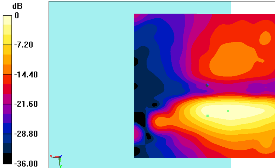
Fig B.3 T-Coil GSM850
