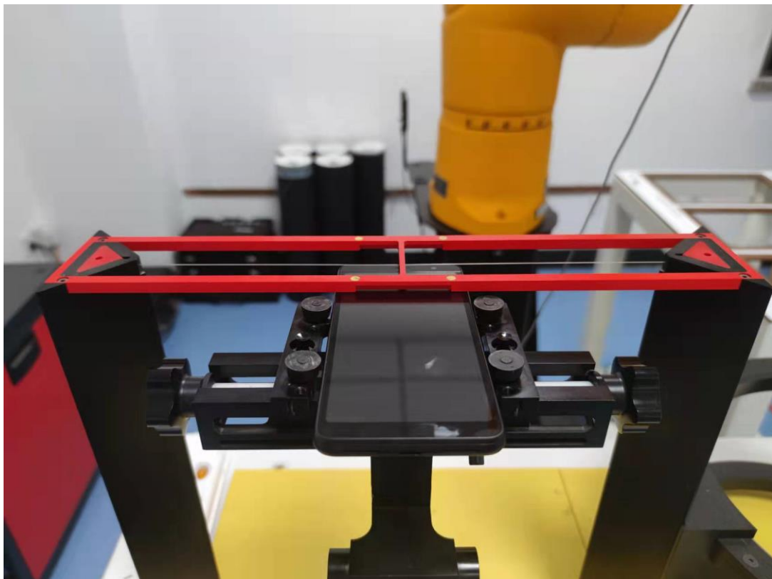
Picture 2: EUT Positioning for RF/T-coil
