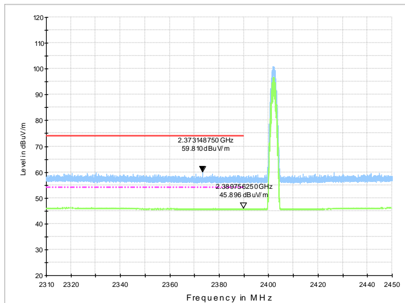
Fig.17. Frequency Band Edges: 8DPSK, Channel 0, 2.31 GHz - 2.45GHz
