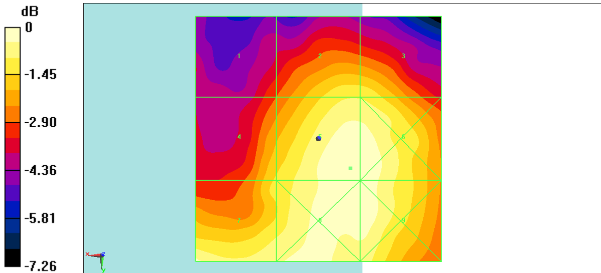
Fig B.3 HAC RF E-Field LTE Band41 Power Class 2 QPSK CH40620
