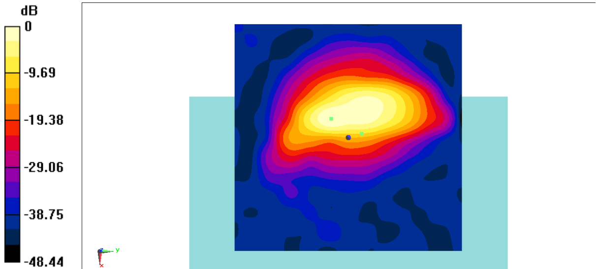
Fig B4 T-Coil GSM850
