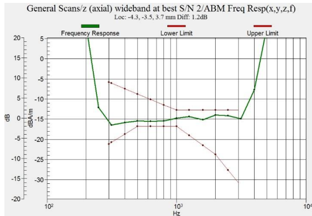
Figure C.2 Frequency Response of EDGE850 – OTT VoIP
