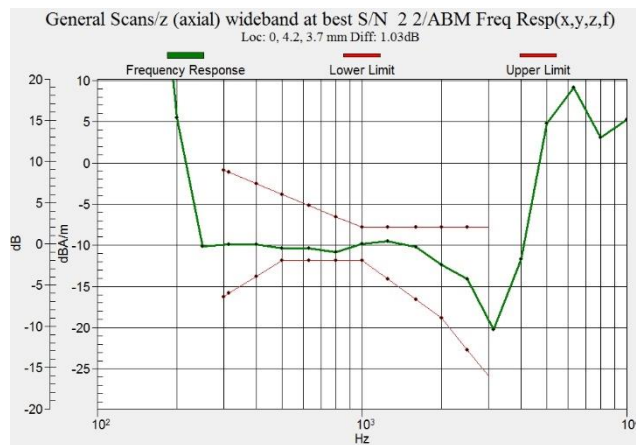
Figure C.5 Frequency Response of WiFi-2.4G
