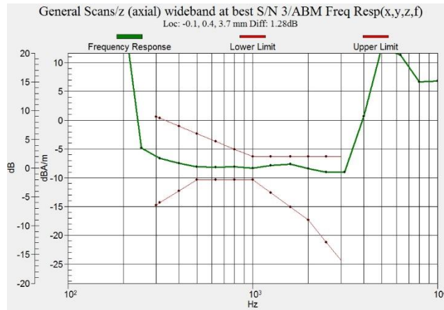
Figure C.4 Frequency Response of LTE B41 PC3
