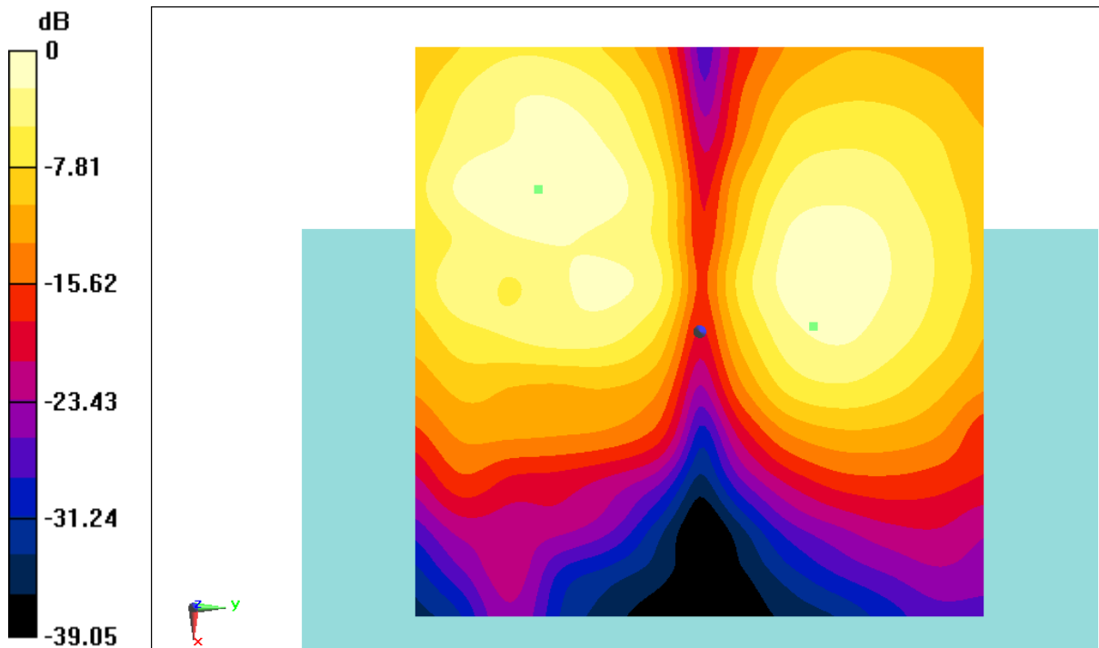
Fig B.17 T-Coil WiFi-2.4G
