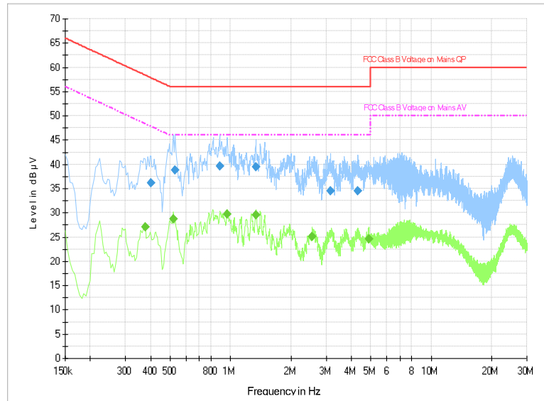
Fig.B.11.2 AC Powerline Conducted Emission-Idle
