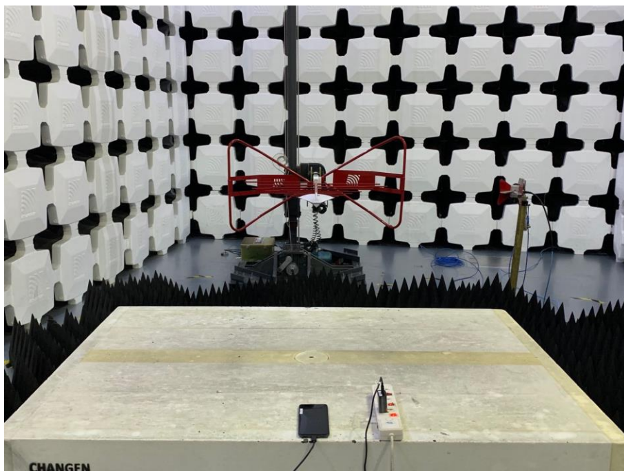
4. Radiated Emissions (Part 15B, Charger+MP4/GNSS/ Camera /GSM idle/WCDMA idle/LTE idle,1GHz-18GHz)
