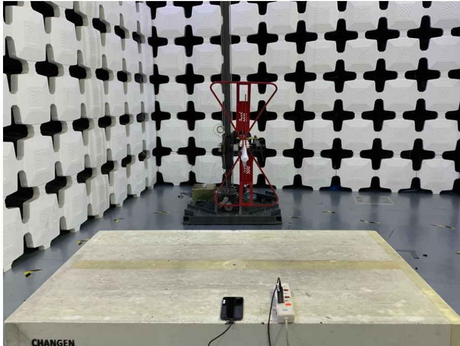
3. Radiated Emissions (Part 15B, Charger+MP4/GNSS/ Camera /GSM idle/WCDMA idle/LTE idle,30MHz-1GHz)
