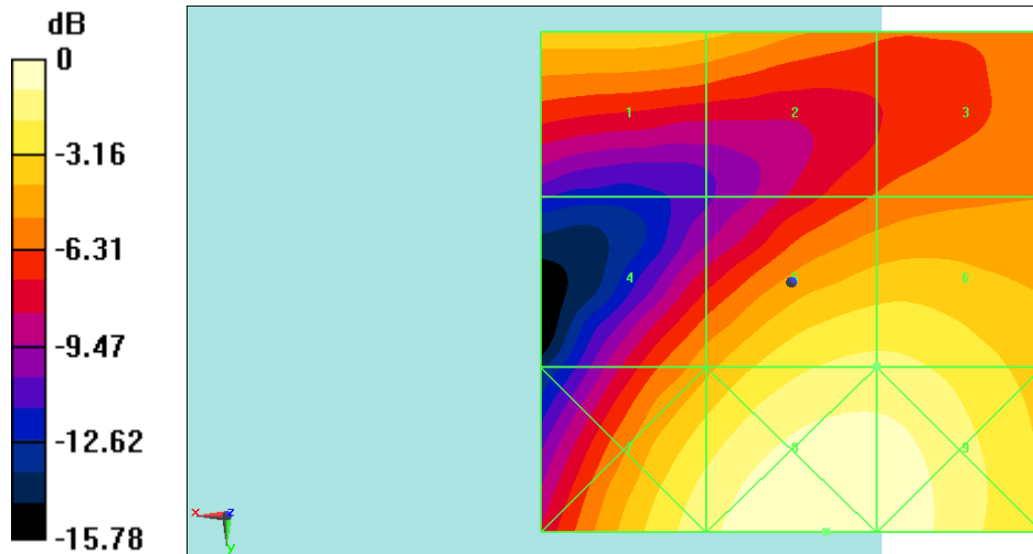
Fig B.2 HAC RF E-Field GSM 1900 Low
