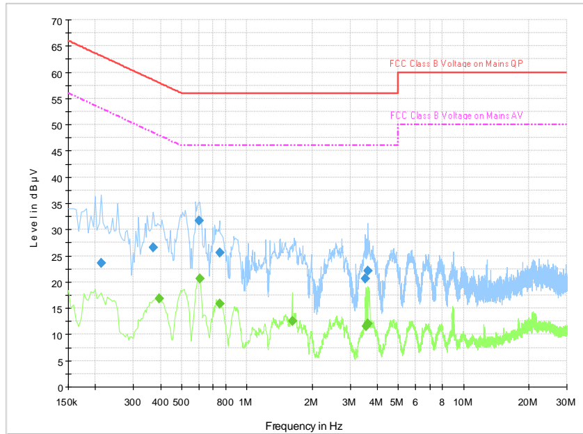
Fig.A.9.1. AC Powerline Conducted Emission- bluetooth
