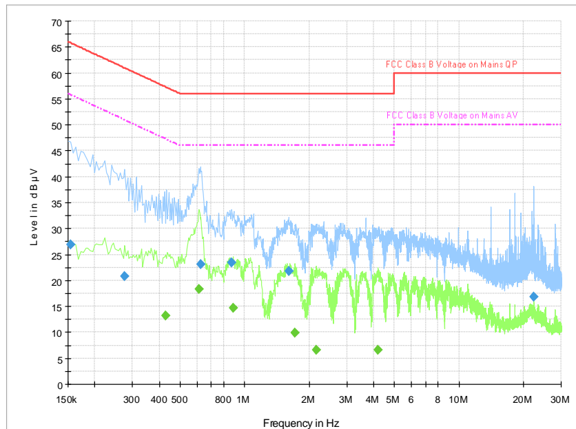
Fig.A.11.1. AC Powerline Conducted Emission- bluetooth
