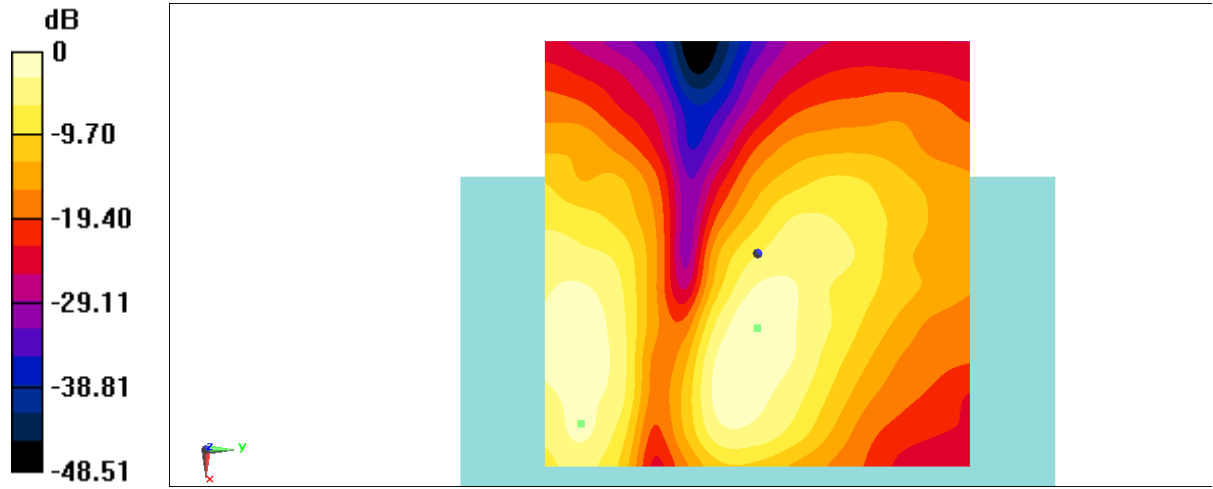
Fig B.3 T-Coil LTE B66
