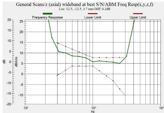
Figure C.2 Frequency Response of LTE B66
