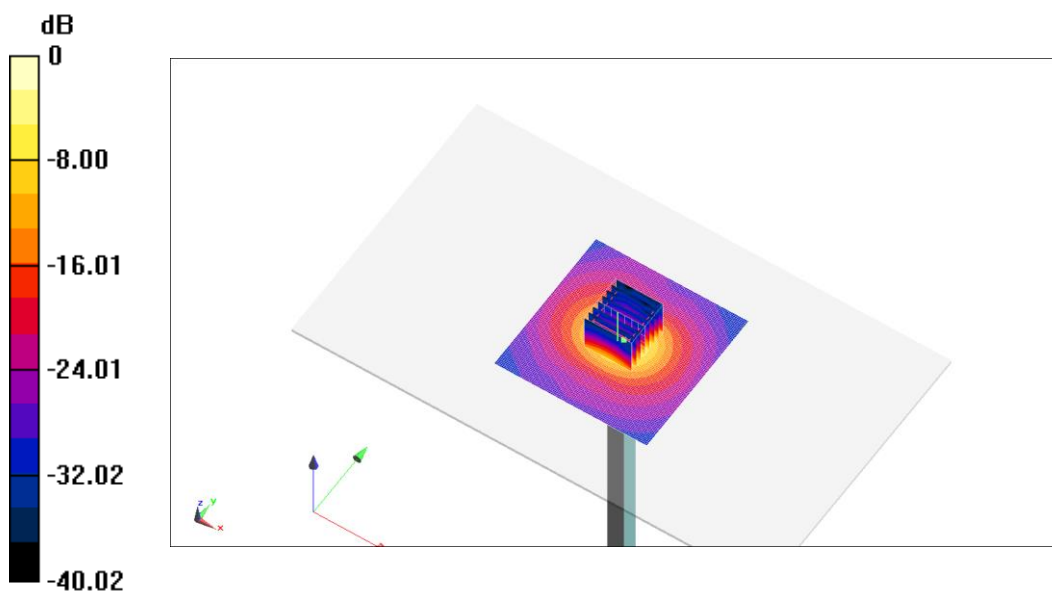
Fig.B.10 validation 5250 MHz 100mW
