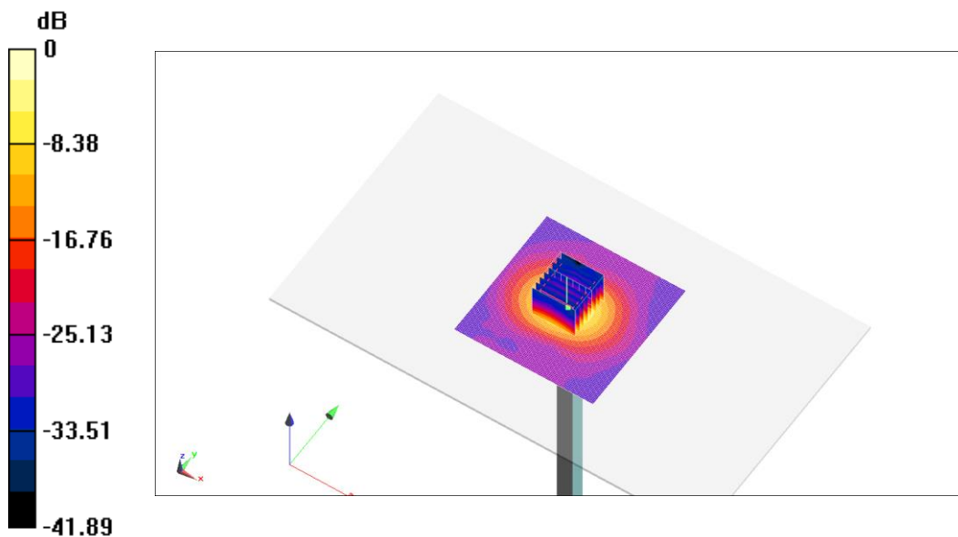
Fig.B.11 validation 5600 MHz 100mW
