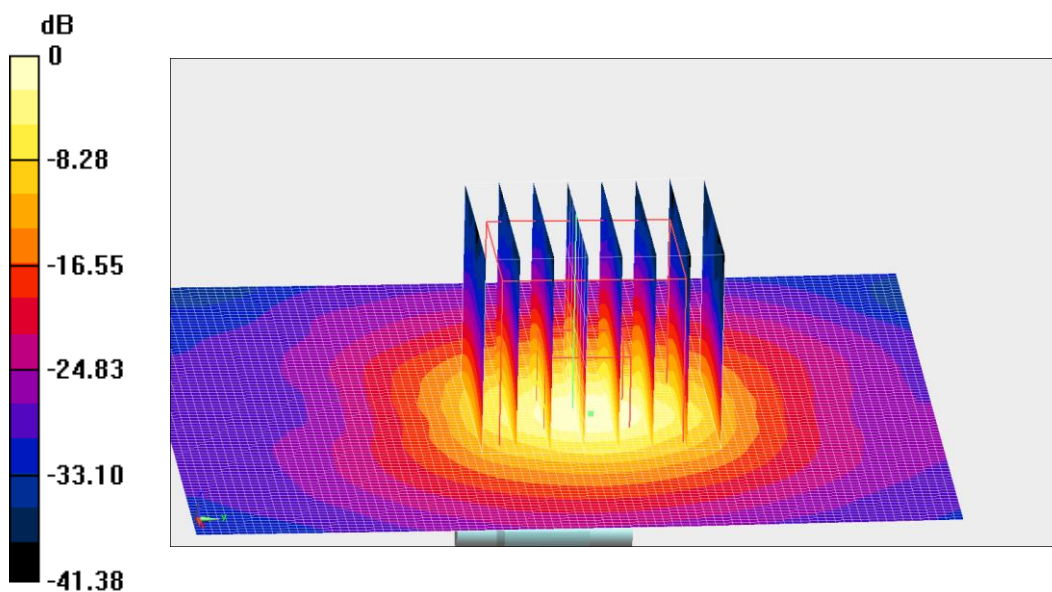
Fig.B.12 validation 5750 MHz 100mW
