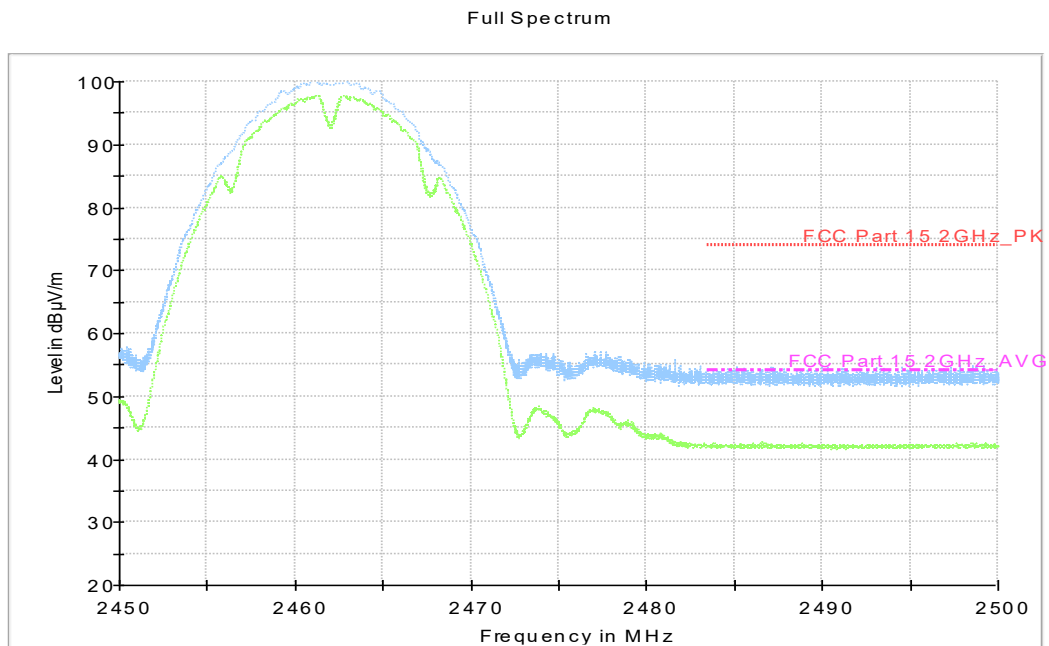
Fig.A.5.2.2 Transmitter Spurious Emission - Radiated Band edge: 802.11b, ch11, 2.45 GHz - 2.50GHz
