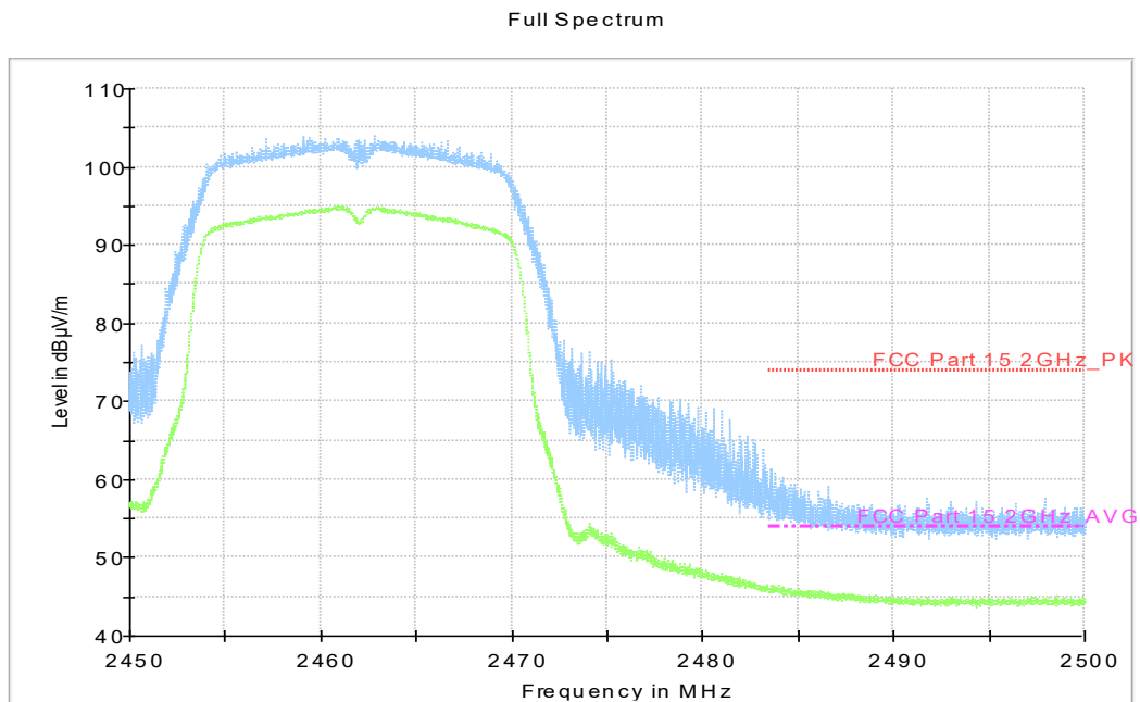
Fig.A.5.2.4 Transmitter Spurious Emission - Radiated Band edge: 802.11g, ch11, 2.45 GHz - 2.50GHz
