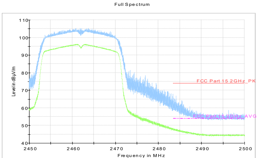
Fig.A.5.2.6 Transmitter Spurious Emission - Radiated Band edge: 802.11n-HT20, ch11, 2.45 GHz - 2.50GHz
