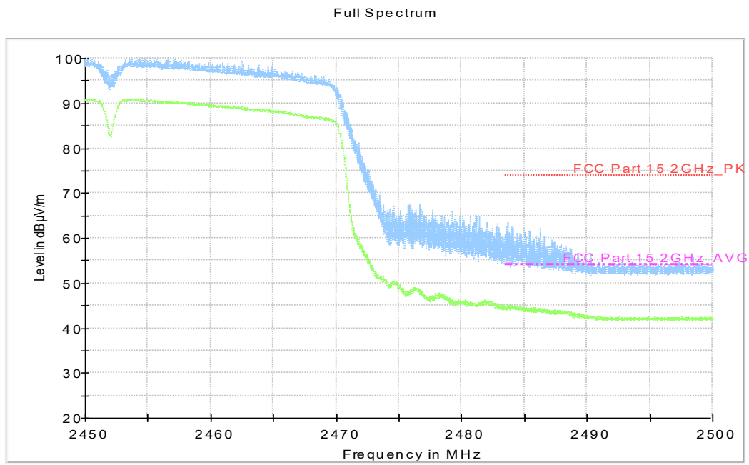
Fig.A.5.2.8 Transmitter Spurious Emission - Radiated Band edge: 802.11n-HT40, ch9, 2.45 GHz - 2.50GHz
