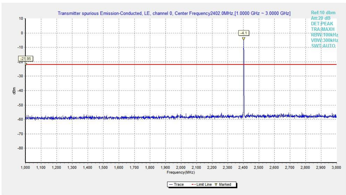
Fig.9. Transmitter Spurious Emission - Conducted: GFSK, 2402 MHz, 1GHz - 3GHz
