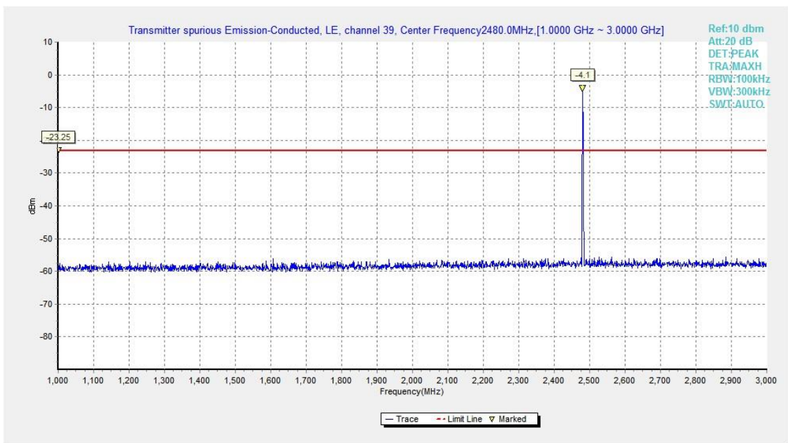
Fig.19. Transmitter Spurious Emission - Conducted: GFSK, 2480 MHz, 1GHz - 3GHz
