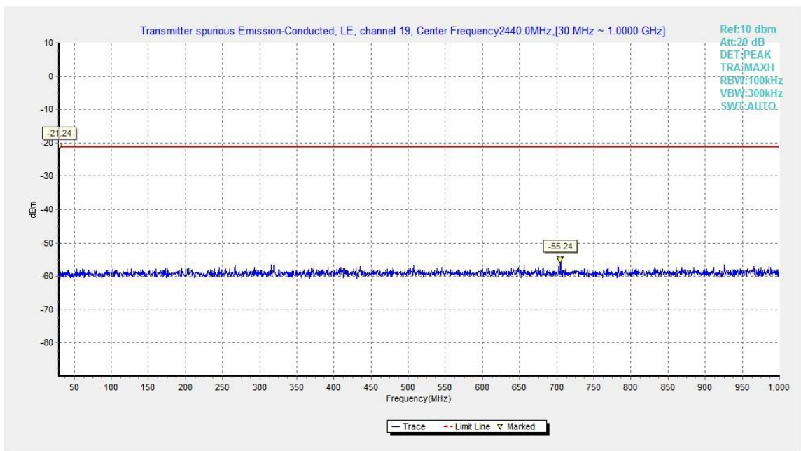
Fig.13. Transmitter Spurious Emission - Conducted: GFSK, 2440 MHz, 30MHz - 1GHz
