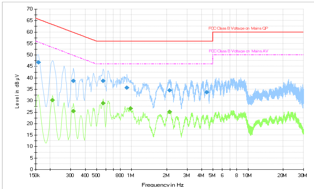
Fig.A.11.2 AC Powerline Conducted Emission EDR-Idle
