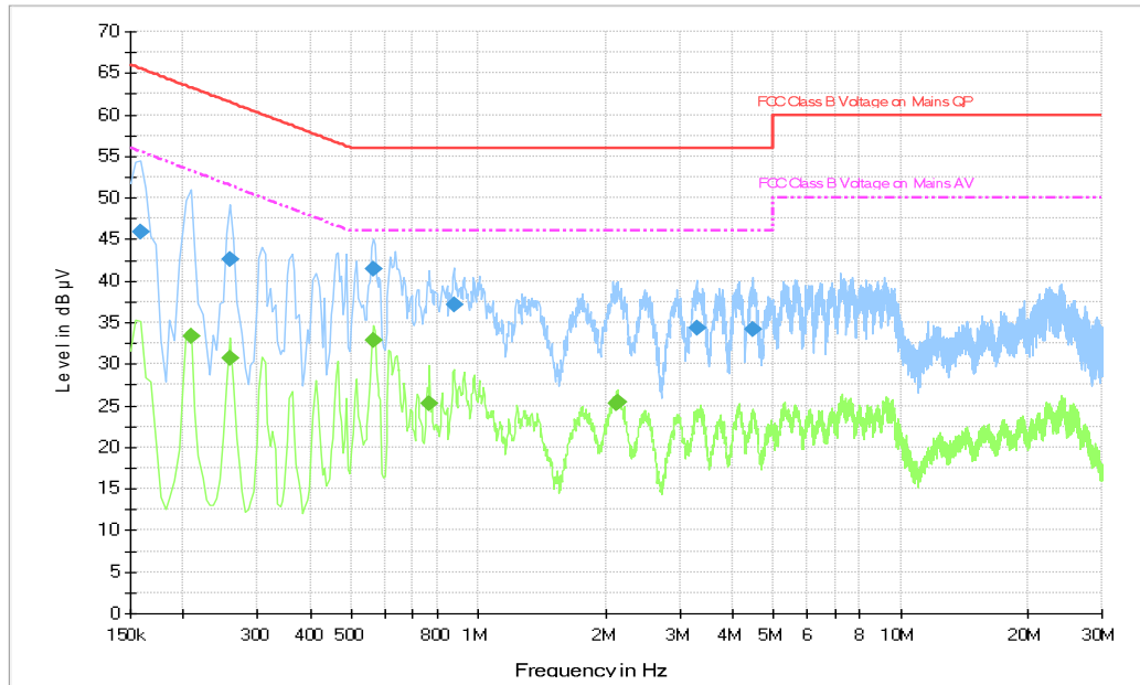
Fig.A.11.1 AC Powerline Conducted Emission-EDR traffic
