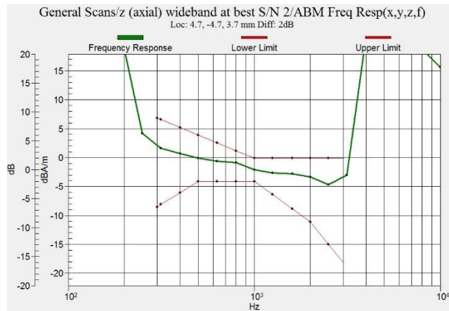
Figure C.5 Frequency Response of EDGE1900 - OTT VoIP
