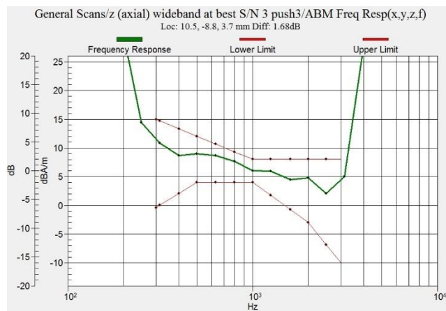
Figure C.6 Frequency Response of LTE B2 - OTT VoIP
