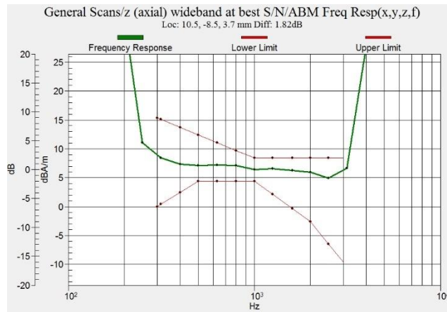
Figure C.8 Frequency Response of WiFi-5G - OTT VoIP
