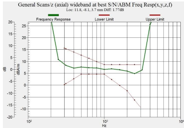
Figure C.4 Frequency Response of WiFi-5G
