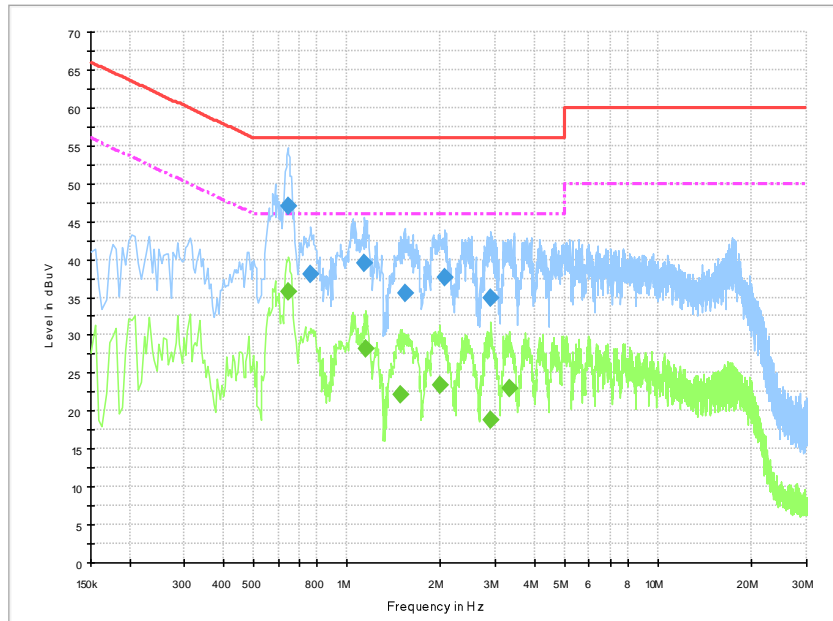
Fig.A.9.1 AC Powerline Conducted Emission-traffic
