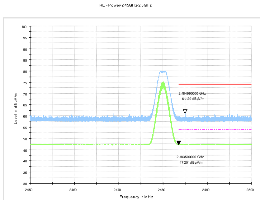
Fig.4. Frequency Band Edges: GFSK, 2480 MHz, 2.45 GHz - 2.50GHz
