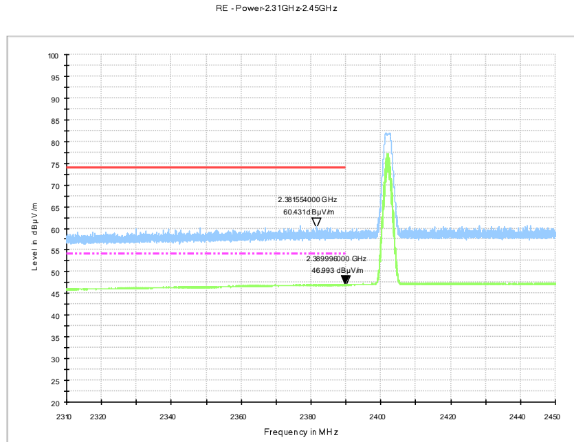
Fig.3. Frequency Band Edges: GFSK, 2402 MHz, 2.31 GHz – 2.45GHz
