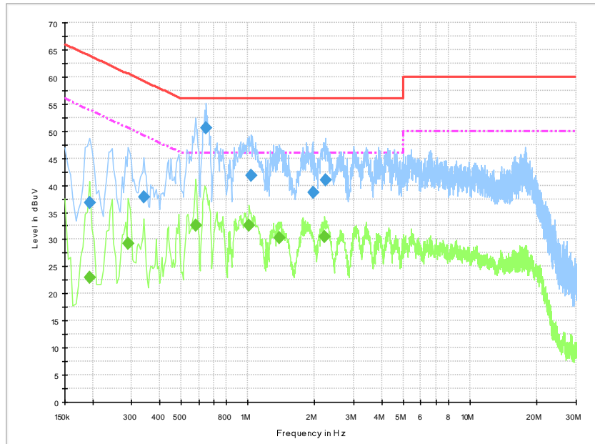
Fig.A.11.2 AC Powerline Conducted Emission-Idle
