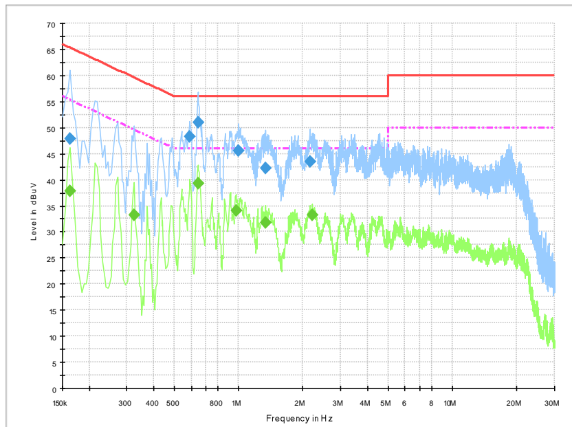
Fig.A.11.1 AC Powerline Conducted Emission-traffic
