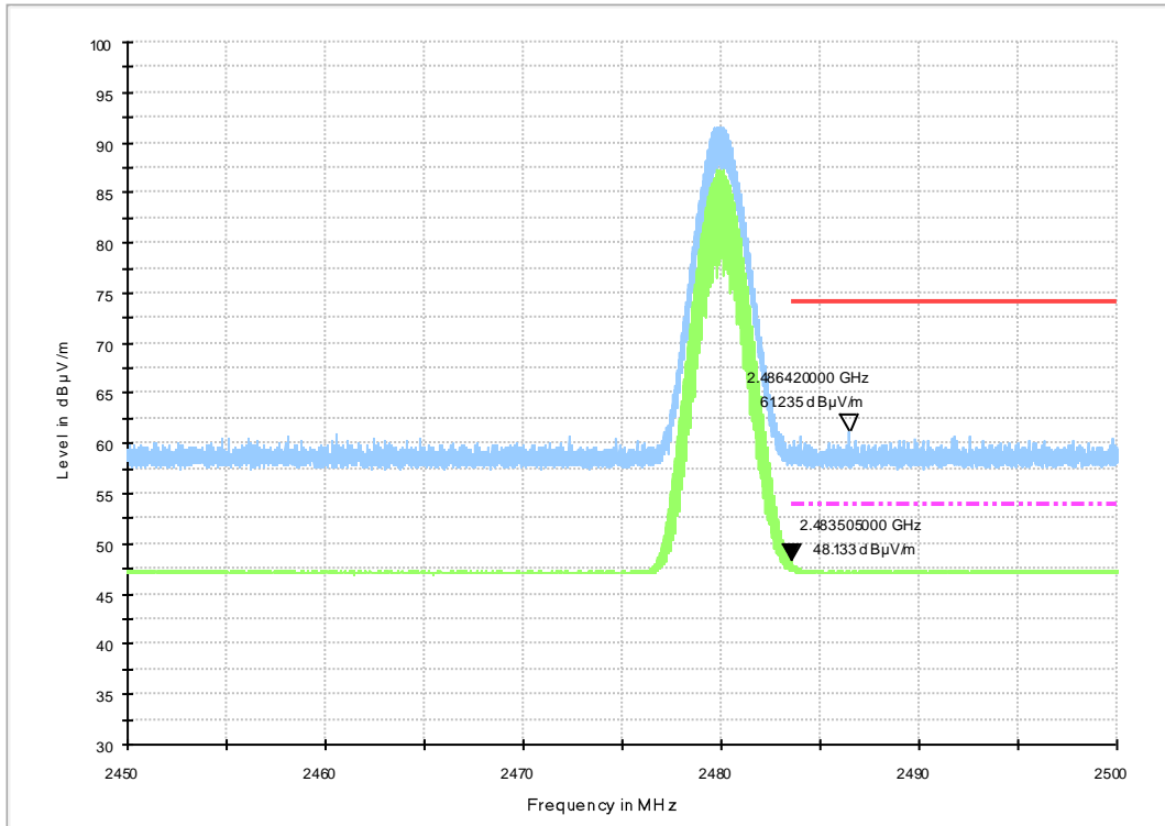
Fig.16. Frequency Band Edges: \pi/4 DQPSK, Channel 78, 2.45 GHz - 2.50GHz
