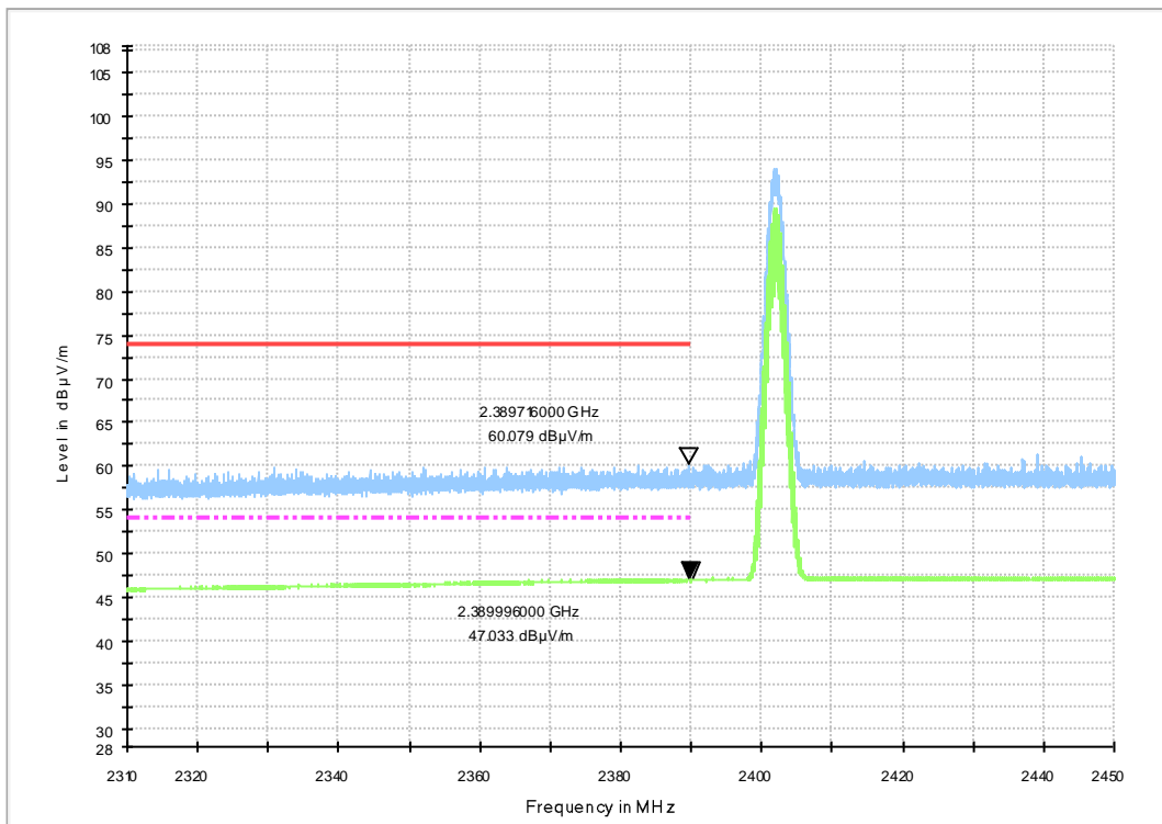
Fig.15. Frequency Band Edges: \pi/4 DQPSK, Channel 0, 2.31 GHz - 2.45GHz
