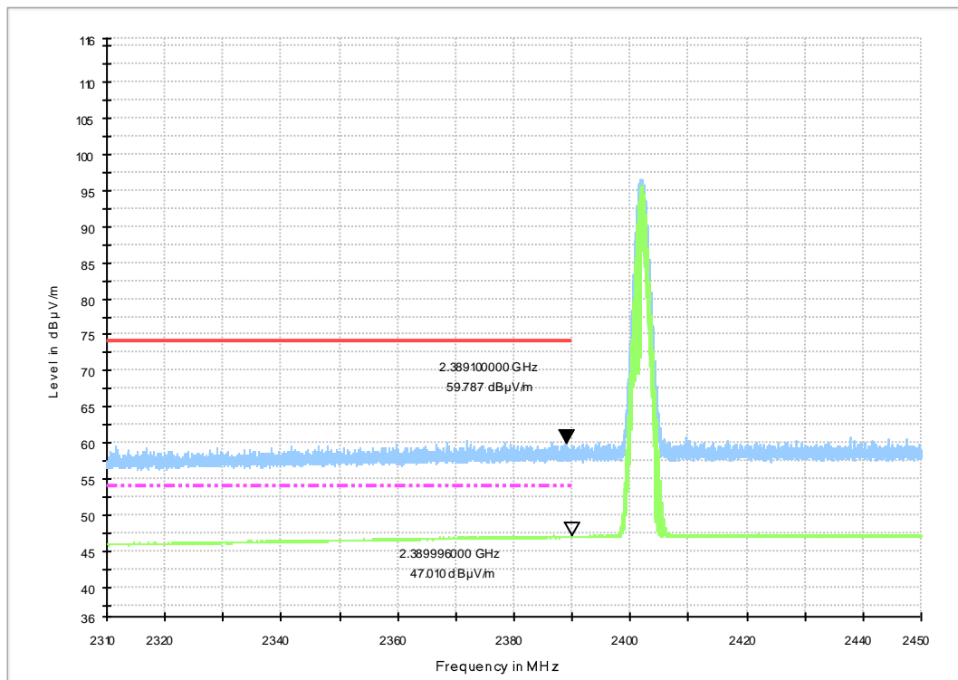
Fig.13. Frequency Band Edges: GFSK, Channel 0, 2.31 GHz – 2.45GHz
