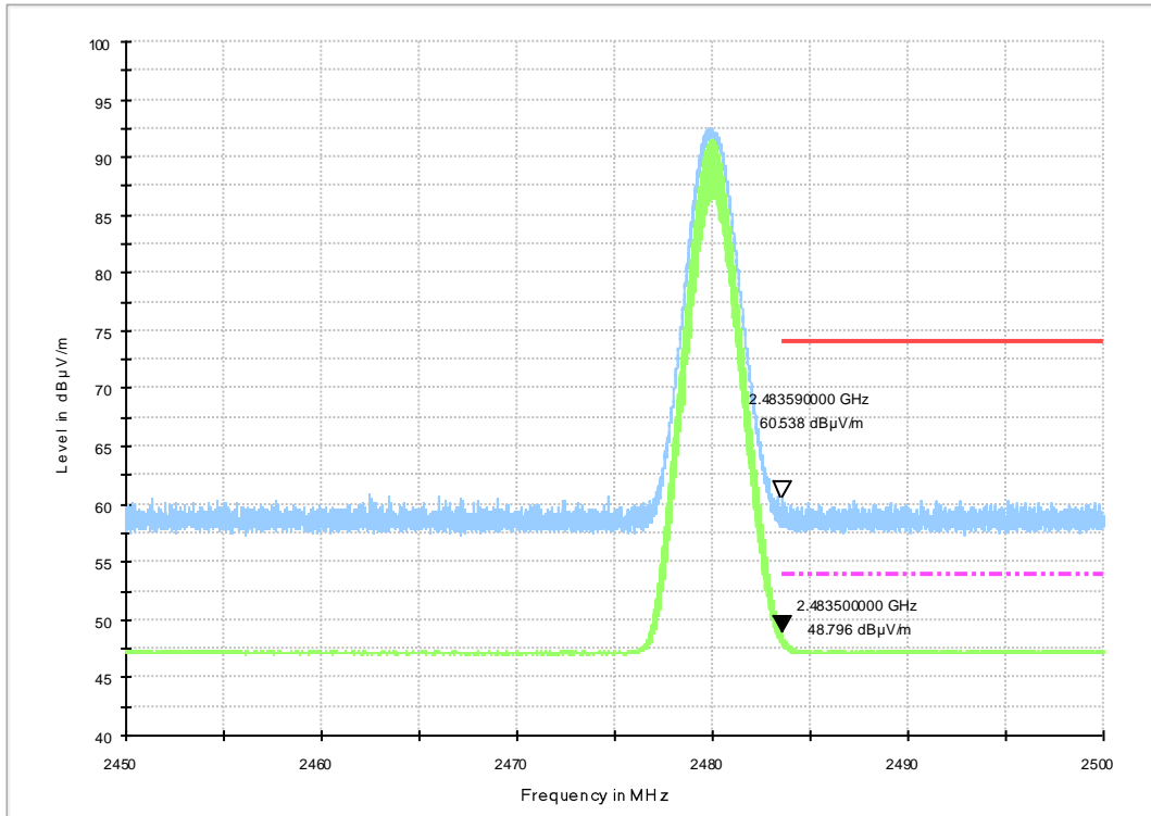
Fig.14. Frequency Band Edges: GFSK, Channel 78, ch11, 2.45 GHz - 2.50GHz
