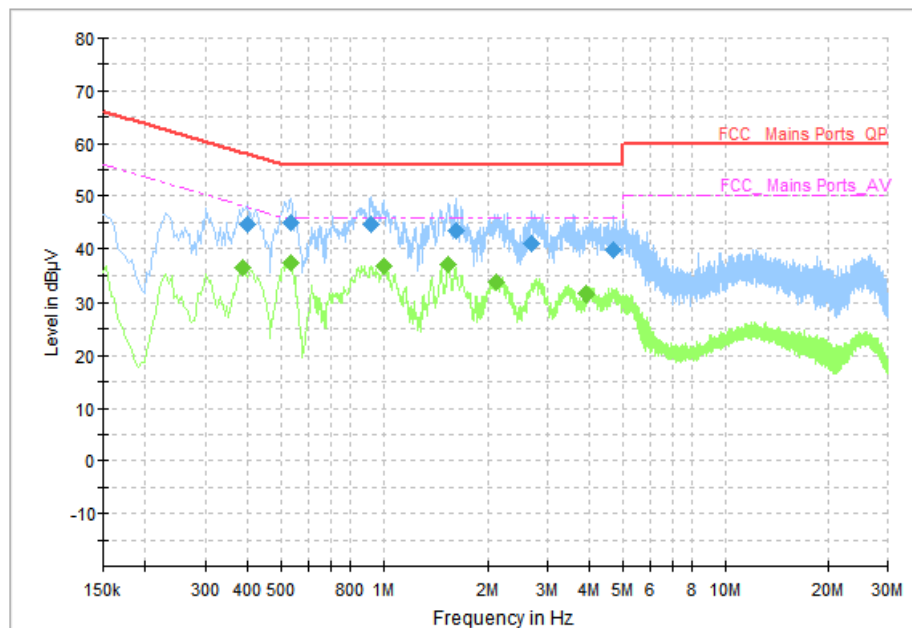
Fig.69 AC Power line Conducted Emission (Idle, AE2, 120V)
