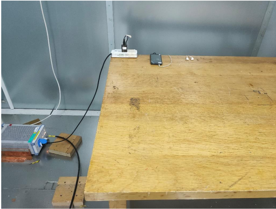
13. Conducted Emission (Part 15B, Charging Mode with FM Mode )
