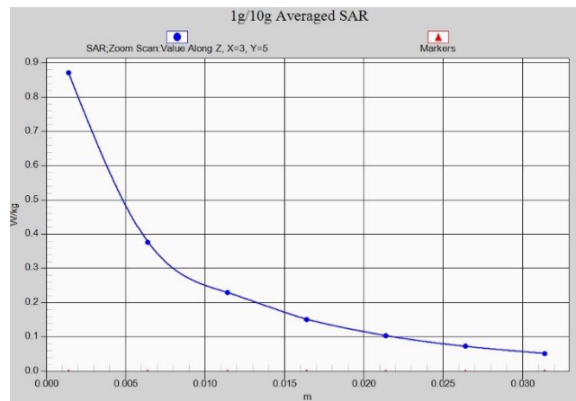
Fig. 1-25 Z-Scan at power reference point (LTE Band71)
