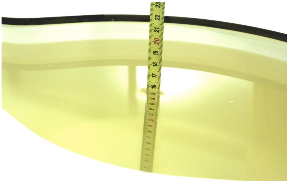
Picture 7-6 Liquid depth in the Flat Phantom (2600MHz)
