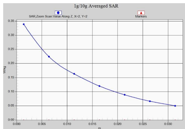
Fig. 1-26 Z-Scan at power reference point (LTE Band71)
