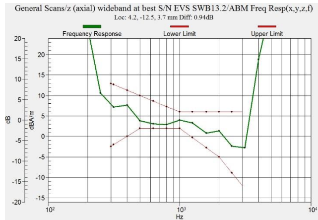
Figure F.6.2 Frequency Response of LTE B5
