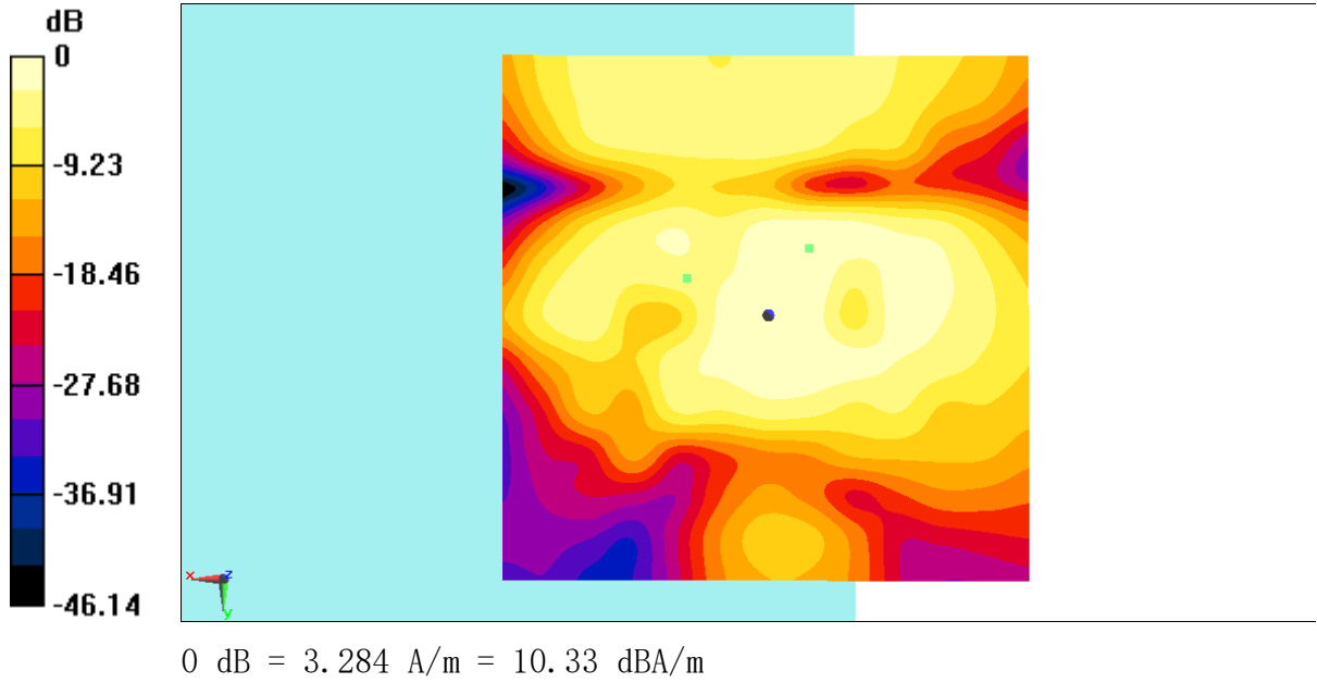
Fig F3.3 T-Coil WCDMA 850
