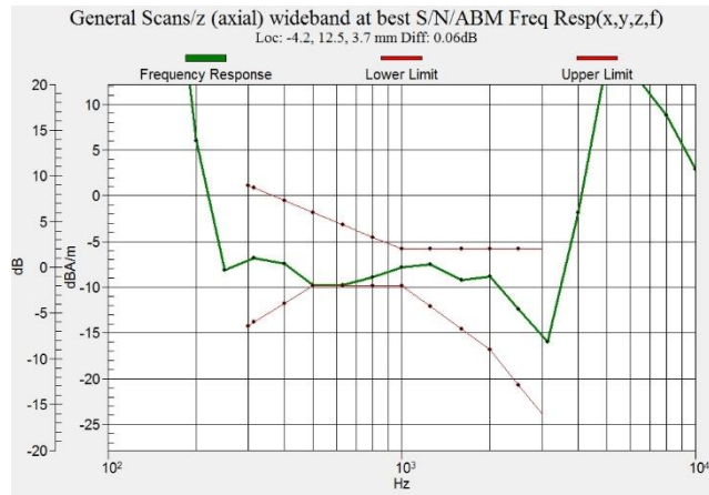
Figure F.5.4 Frequency Response of WiFi 2.4G
