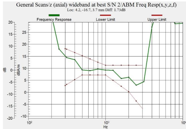
Figure F.5.1 Frequency Response of GSM 850
