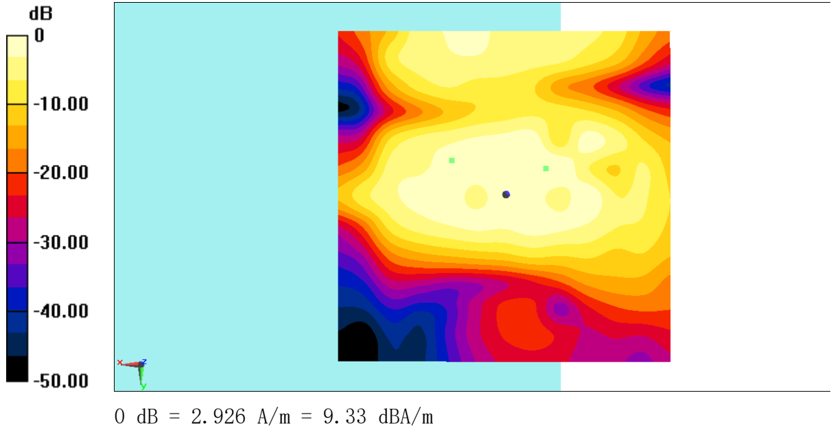
Fig 4.5 T-Coil LTE B7
