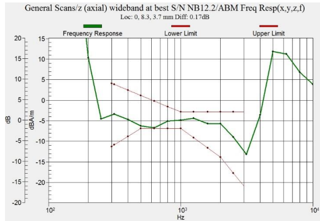
Figure F.6.1 Frequency Response of LTE B2
