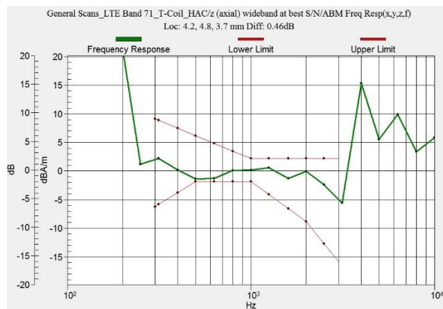
Figure C.9 Frequency Response of LTE B71
