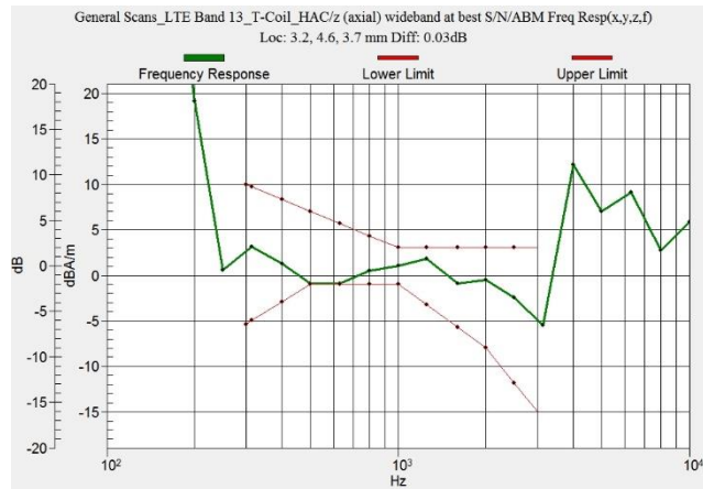
Figure C.7 Frequency Response of LTE B13
