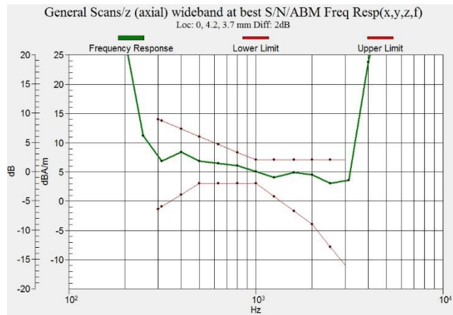
Figure C.11 Frequency Response of EDGE 1900 - OTT VoIP
