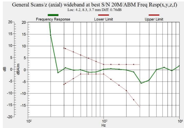
Figure C.13 Frequency Response of LTE B66 - OTT VoIP
