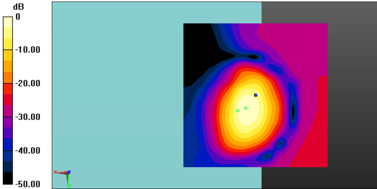
Fig B.14 T-Coil LTE B13
