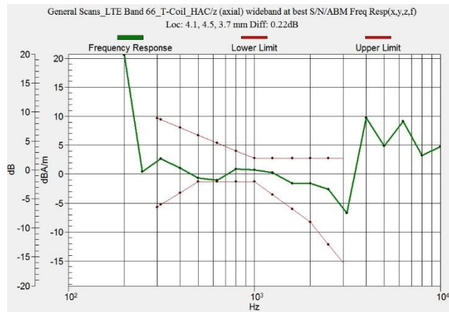
Figure C.8 Frequency Response of LTE B66
