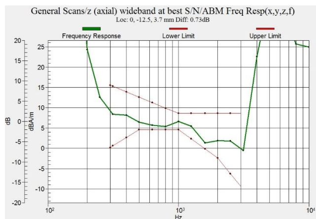
Figure F.6.3 Frequency Response of LTE B7
