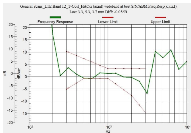
Figure C.6 Frequency Response of LTE B12
