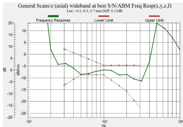
Figure F.5.2 Frequency Response of WCDMA 850
