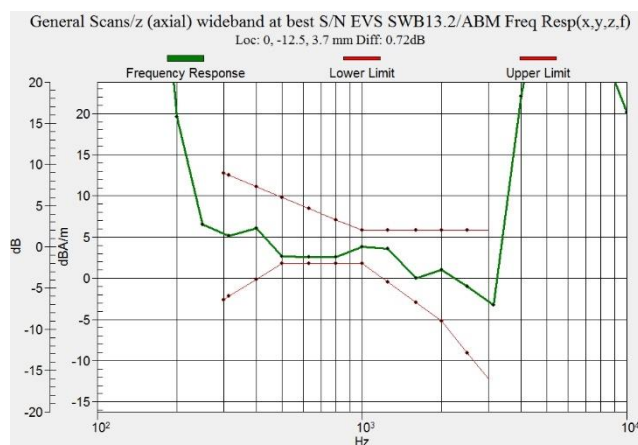
Figure F.5.3 Frequency Response of LTE B66
