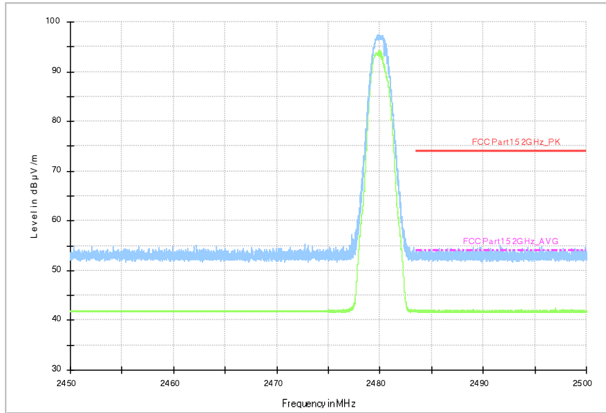
Fig.18. Frequency Band Edges: 8DPSK, Channel 78, 2.45 GHz - 2.50
