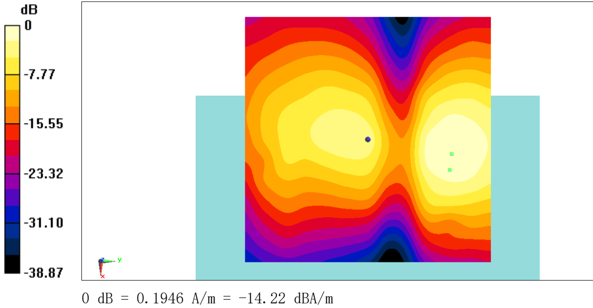
Fig B.3 T-Coil LTE B13
