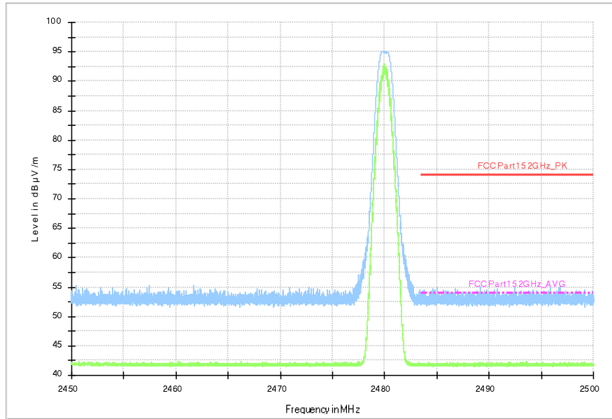
Fig.4. Frequency Band Edges: GFSK, Channel 39, 2.45 GHz - 2.50GHz
