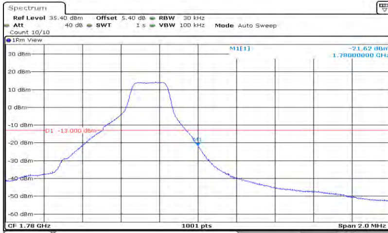
Band66-1.4MHz-16QAM-132665-6RB#0
