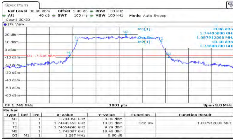
Band66-1.4MHz-QPSK-132322-6RB#0-1.088
