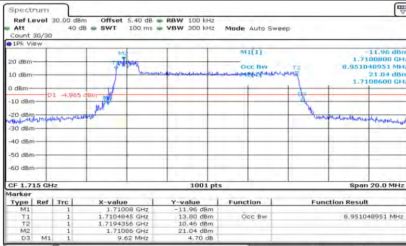
Band66-10MHz-16QAM-132022-50RB#0-8.951
