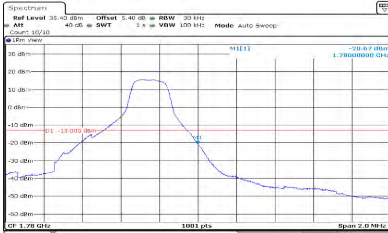
Band66-1.4MHz-QPSK-132665-6RB#0
