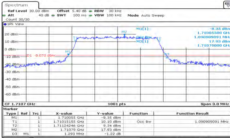
Band66-1.4MHz-QPSK-131979-6RB#0-1.091
