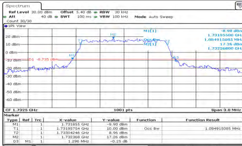
Band4-1.4MHz-QPSK-20175-6RB#0-1.085
