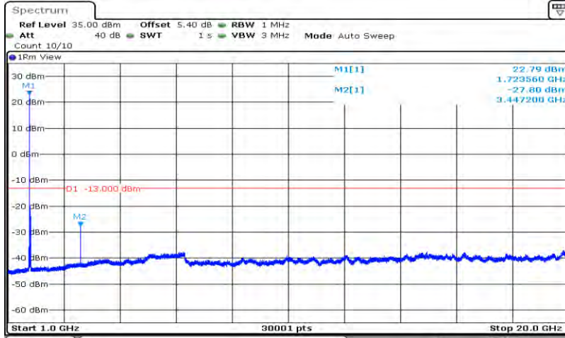
Band4-20MHz-16QAM-20175-1RB#0-Range2:1000~20000MHz
