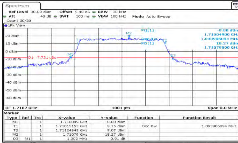
Band4-1.4MHz-QPSK-19957-6RB#0-1.094
