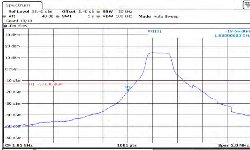
Band2-1.4MHz-16QAM-18607-6RB#0
