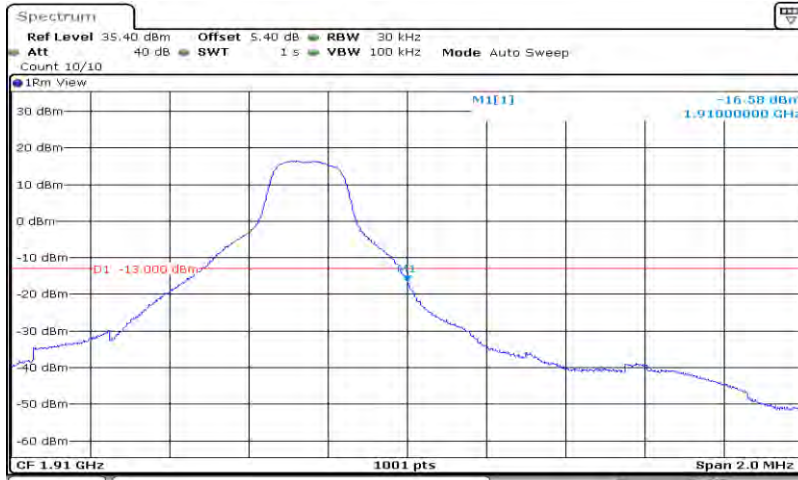
Band2-1.4MHz-QPSK-19193-6RB#0
