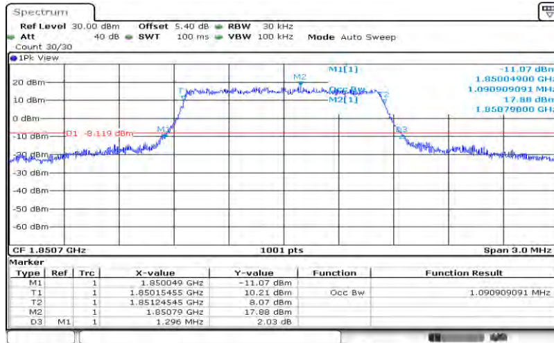
Band2-1.4MHz-QPSK-18607-6RB#0-1.091
