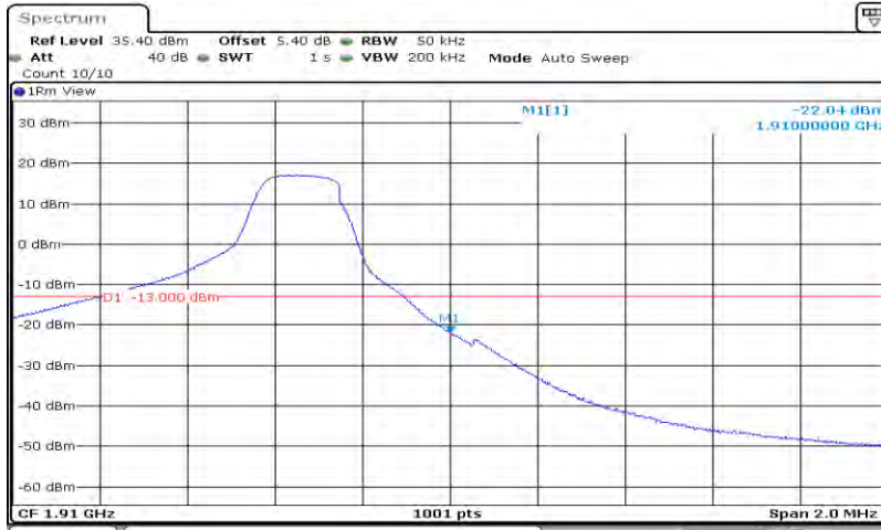
Band2-5MHz-16QAM-19175-25RB#0
