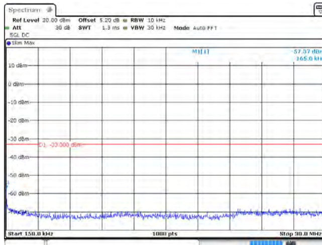
EGPRS1900_512
