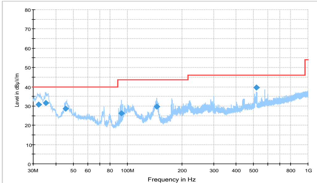
Figure A.14 Radiated Emission from 30MHz to 1GHz
